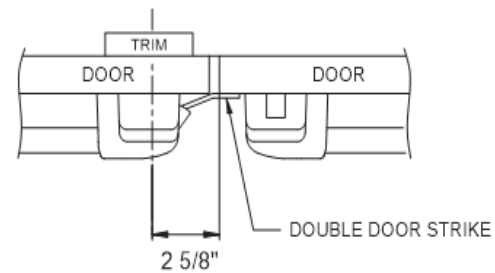
C. DOUBLE DOOR WITHOUT MULLION
